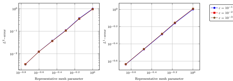
Fig. 1 Numerical results for the RS-IMEX scheme (left) and the Dolejší-Feistauer-Kučera scheme (right); errors are in density and momentum. It can be seen that the errors are apparently independent of \varepsilon , which is typically a good indicator for a scheme being asymptotically consistent. Errors and mesh sizes have been scaled (independently on \varepsilon ), so that they begin at (1, 1). To account for the dimensions in the Dolejší-Feistauer-Kučera scheme, error in density is scaled by \varepsilon^{-2} . Please note that quantities on the left and on the right cannot be compared right away.
