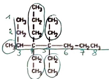
4,5,5-triethyl-3-methyl-4-propyloctane
