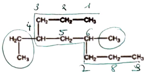
4-ethyl-6-methylnonane
