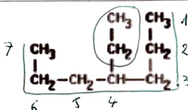
4-ethylheptane
