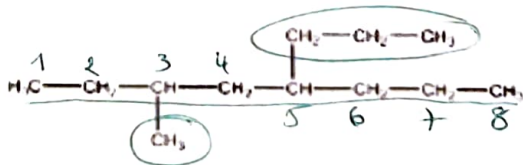
3-methyl-5-propyloctane
