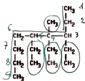
3,4,5-triethyl-4-methylnonane
