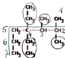
4,4-diethyl-2,3-dimethylheptane
