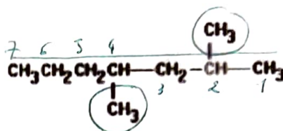
2,4-dimethylheptane
