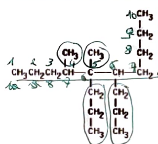
4,5-dimethyl-5,6-dipropyldecane
