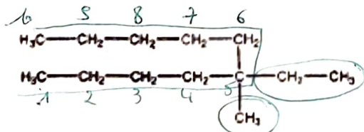
5-ethyl-5-methyldecane
